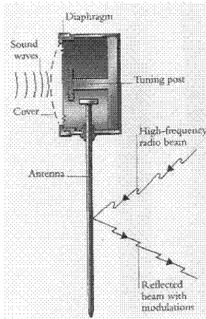
The cavity resonator hidden inside the Great Seal had no wires, no conventional microphone, and no batteries. (Diagram from H. Keith Melton, The Ultimate Spy Book . (New York: DK Publishing, Inc., 1996). (C))
