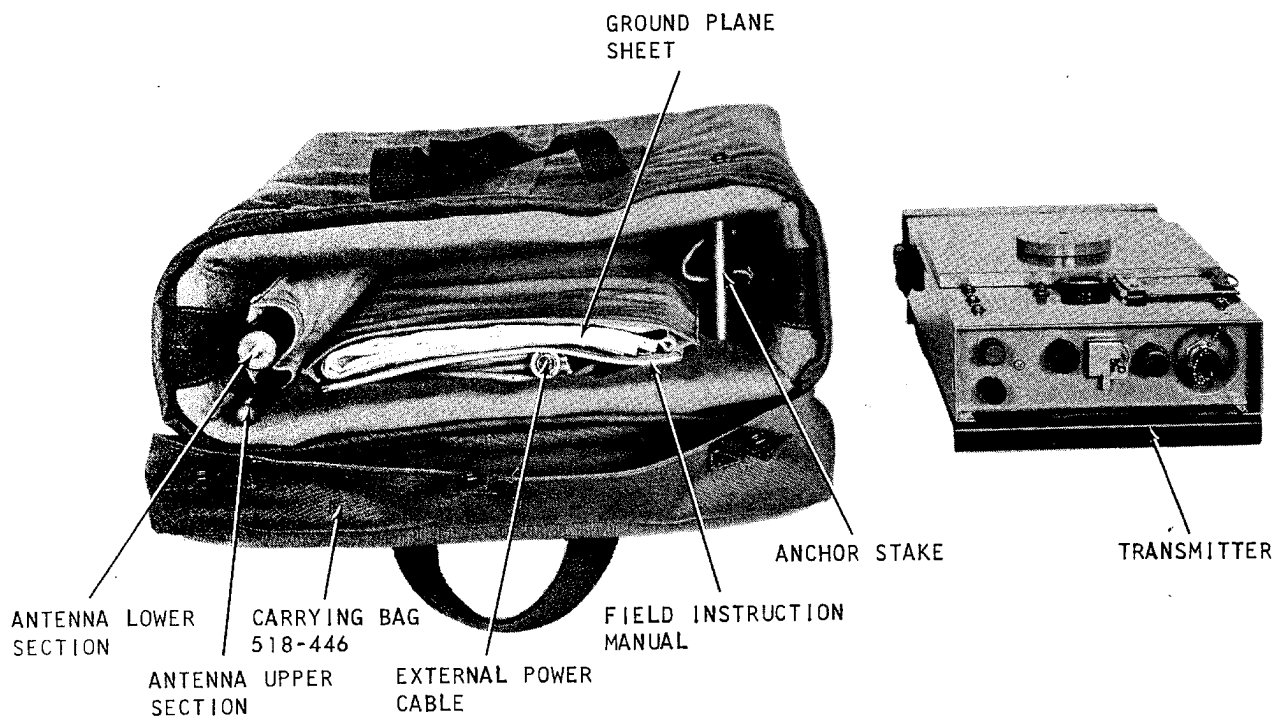
Figure 1. HRT-2C Beacon Transmitter
