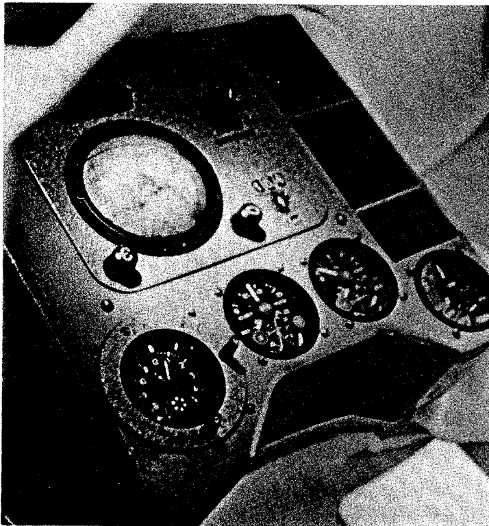
Figure 39. Vostok instrument panel, showing globe reference instrument.
