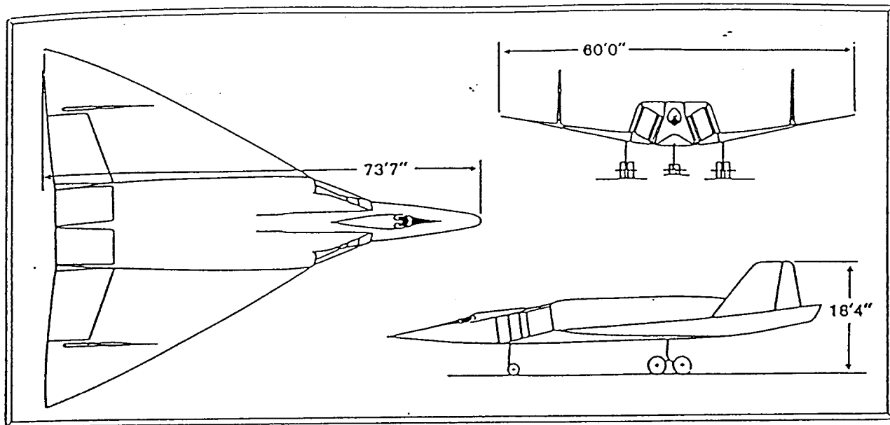
Convair KINGFISH
