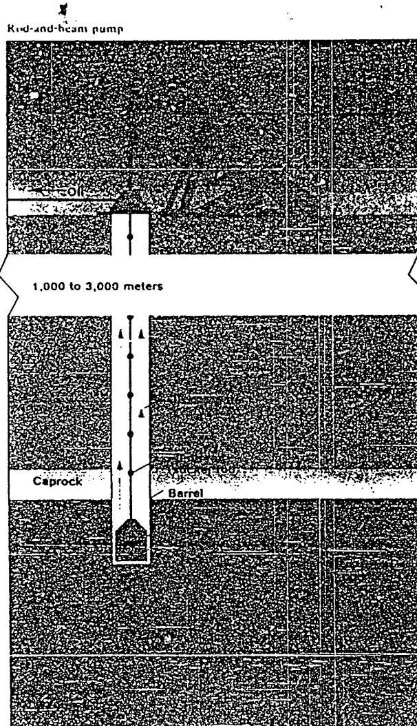
Figure 3 Artificial Lift Equipment
