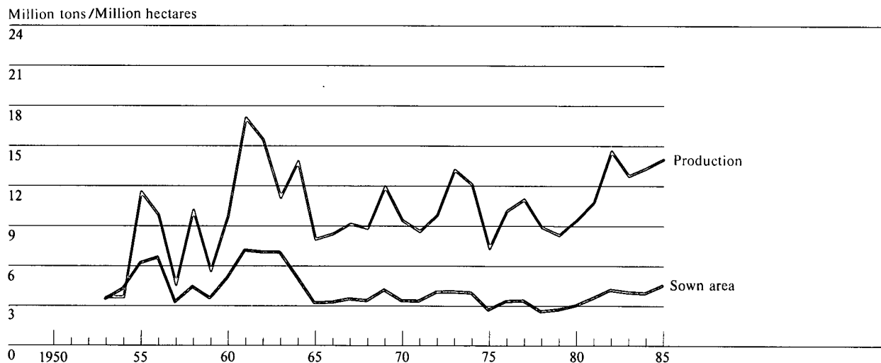
Figure 3 USSR: Corn Grain Trends, 1950-85 a
