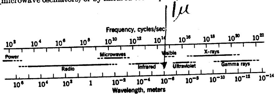
Fig. 40-1 The electromagnetic spectrum. Note that the wavelength and frequency scales are logarithmic.
