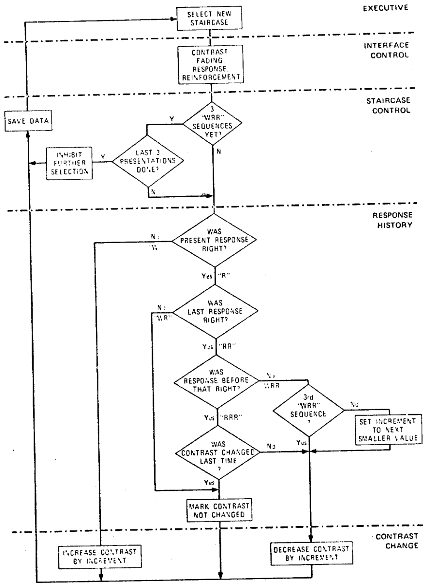
Fig. 7. Flow-chart representation of the FCS computer program.
