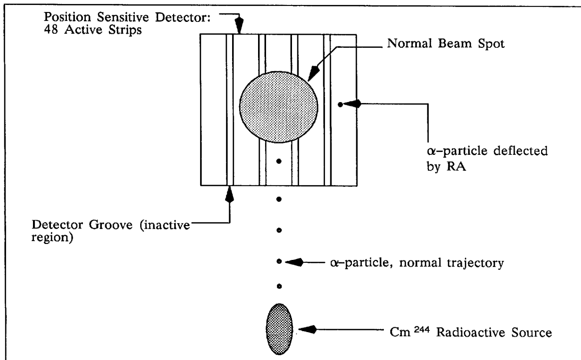
FIGURE 1 CONCEPTUAL CONFIGURATION OF AN \alpha -PARTICLE EXPERIMENT
