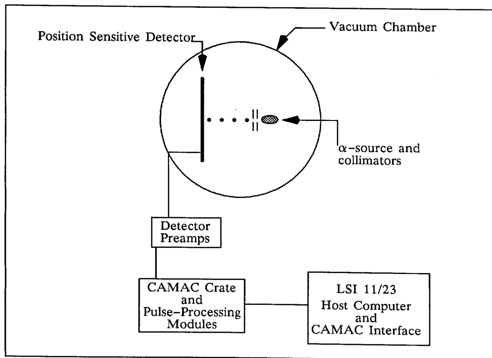
FIGURE 2 SINGLE \alpha -PARTICLE RA APPARATUS
