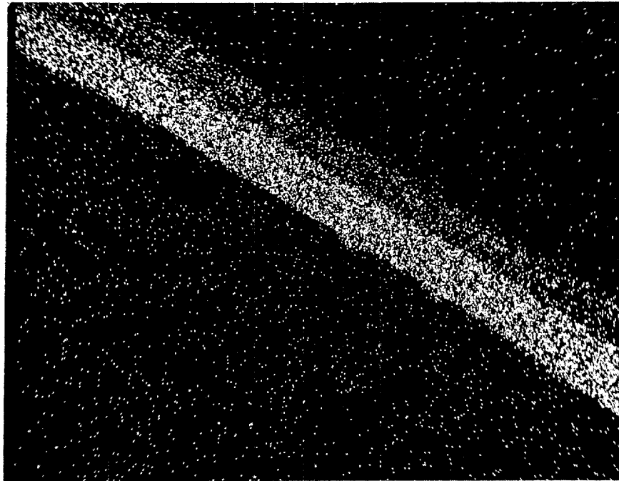
Figure 30. SEM-X Zinc X-ray Map of Control Cross-Section
