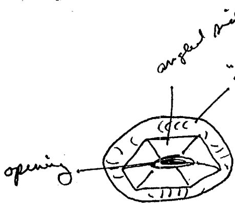
Fractal view
