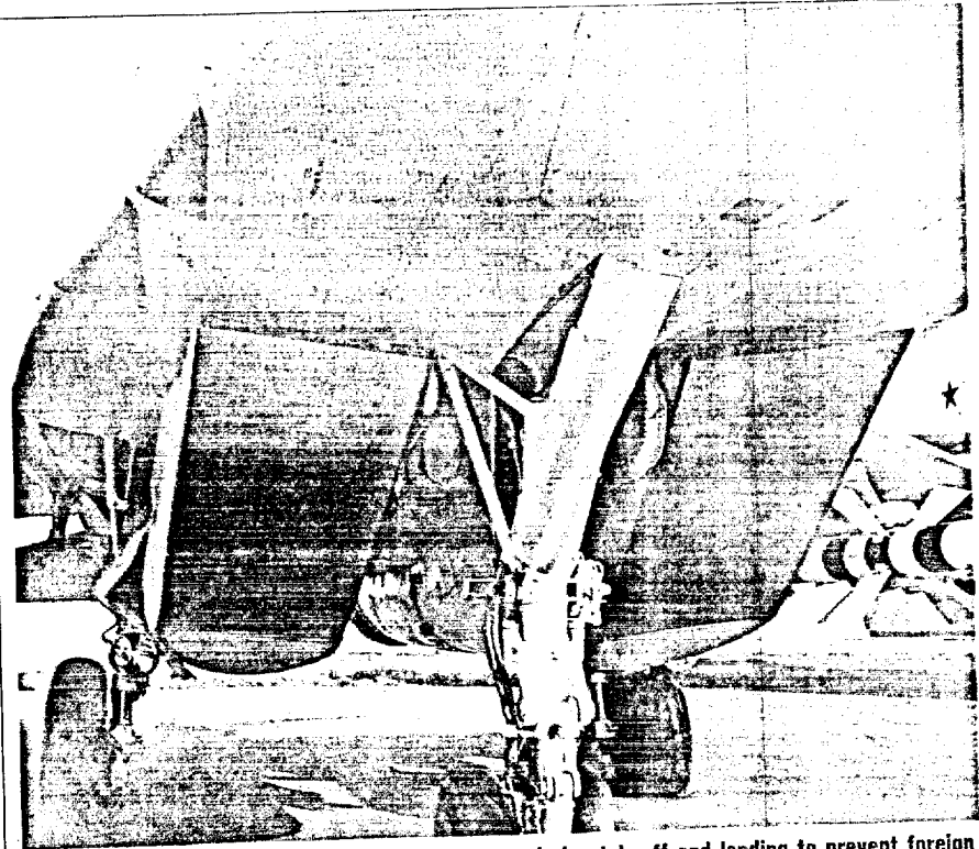
MiG-29 engine air intakes feature doors that close during takeoff and landing to prevent foreign object ingestion. Engine air is taken in through louvers in upper surface of wing root leading edge.
