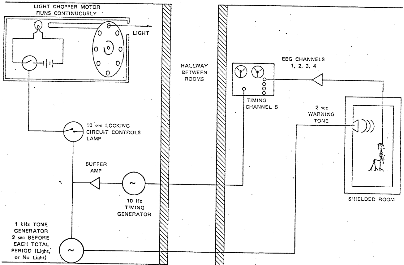
FIGURE 1 REMOTE SENSING EEG EXPERIMENT
