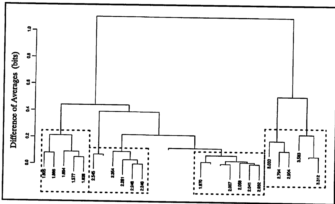
Figure 6. Cluster Diagram for Dynamic Targets
