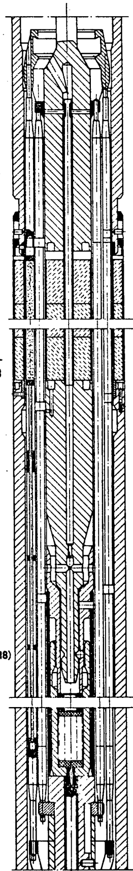
FUEL CHANNEL
