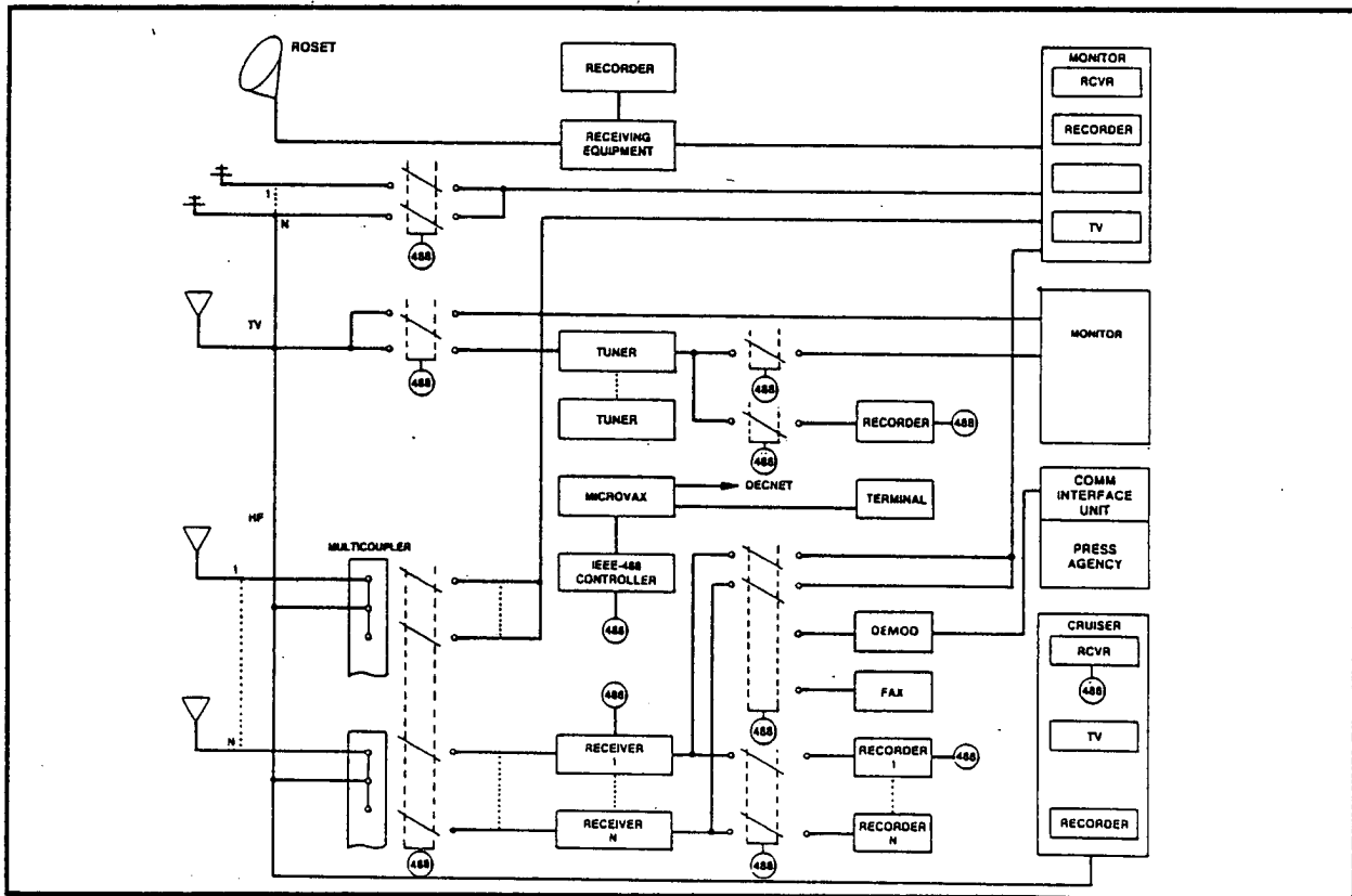
Figure 2-8 Collection Subsystem
