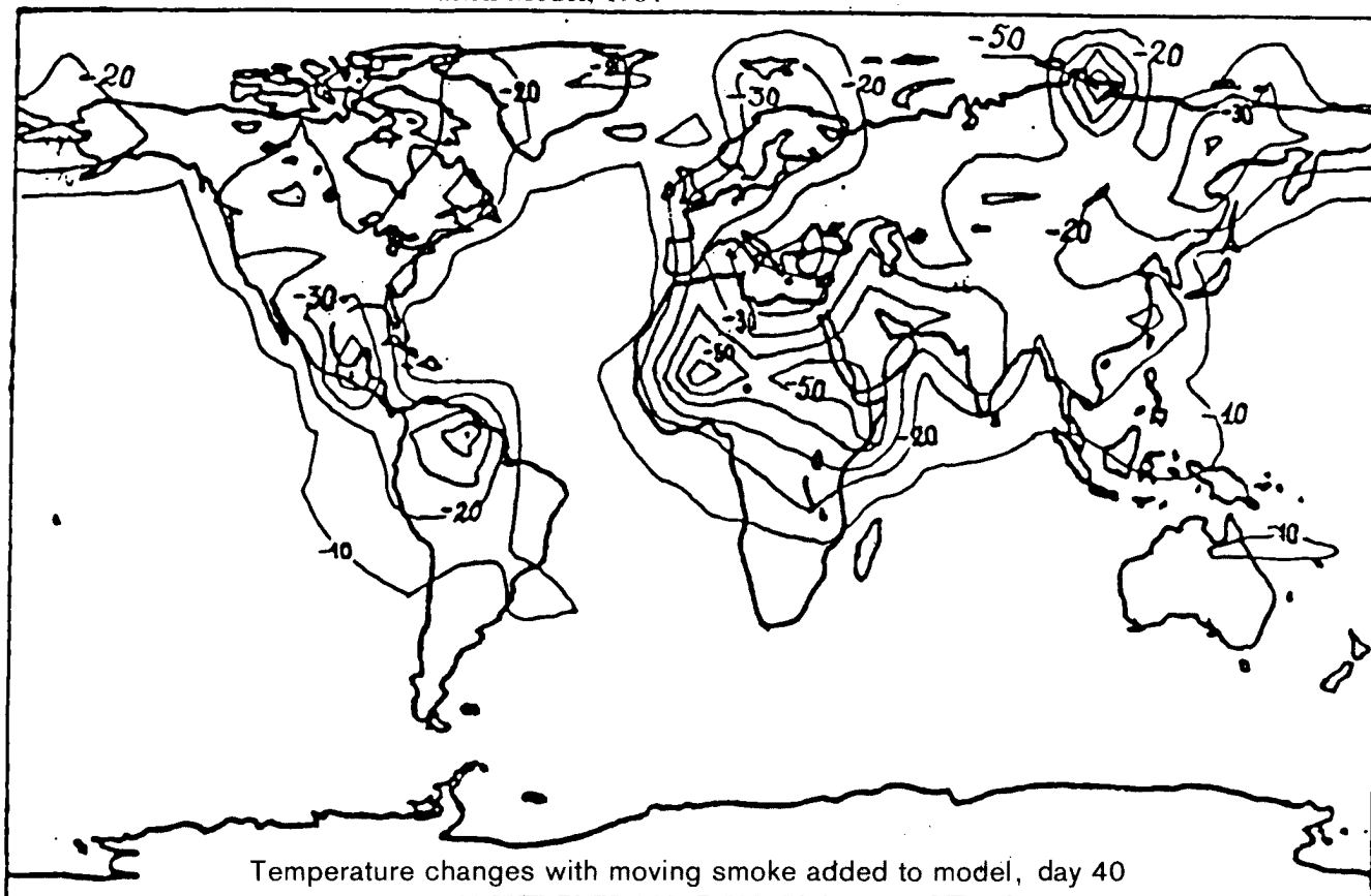
Figure 7 Soviet Nuclear Winter Research: Three-Dimensional Global-Circulation Model, 1984
