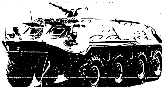
BTR 60PB armored personnel carrier
