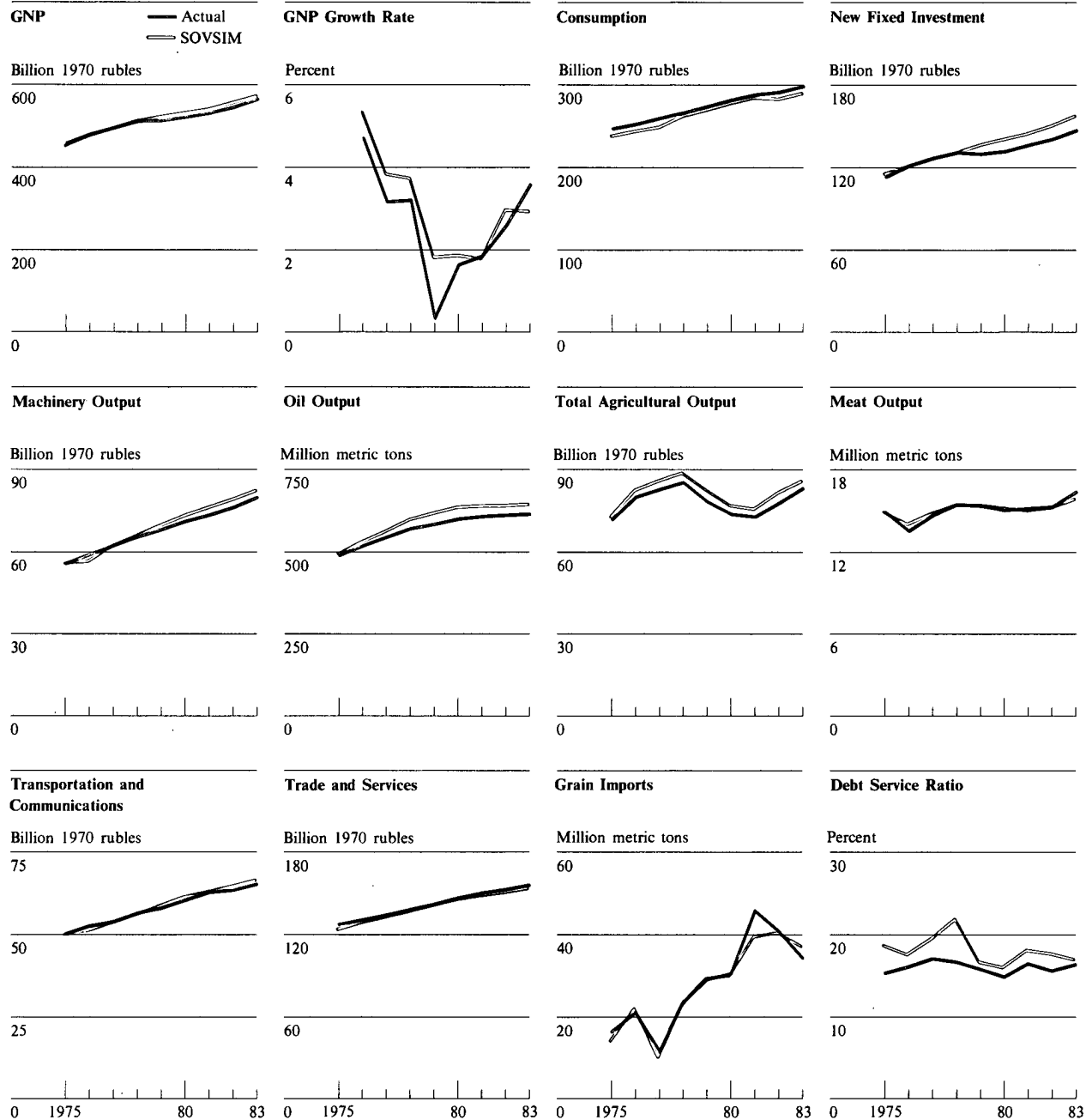
Figure 10 Comparison of 1975-83 SOVSIM Output for Key Variables With Corresponding Actual Values
