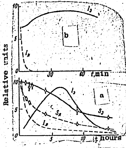
Figure caption: a - time variation of loss of the emission sum S_e and the light sum S_l at 40°C; deduced variation of the afteremission I_e and afterglow I_l . b - curves for I_e and I_l obtained in preliminary experiments employing a new vacuum setup.
