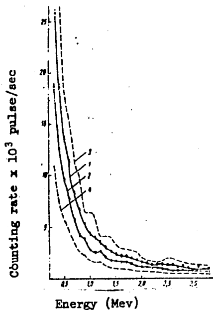
Fig. 1. Gamma-ray spectra obtained by Luna 10 while in orbit around the Moon and along the trajectory of the flight from the earth to the Moon
