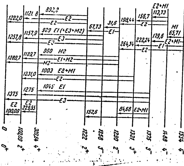
Excited levels of W 182
