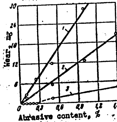
Fig. 2. Wear by weight of steel roller versus size and concentration (wt %) of abrasive particles in lubricant: 1 - 80μ; 2 - 50μ; 3 - 2-3μ.
