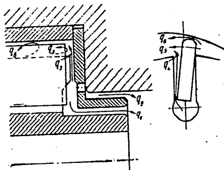
Fig. 2: The paths of leakage in the LLF vane pump. ( q_3 the path of highest leakage)
