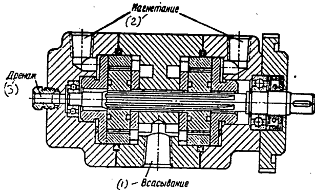
Fig. 4: Dual G12-2 and G12-4 design. (1) - Intake; (2) - pressure; (3) - drain.
