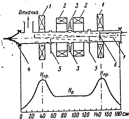
Fig. 1. Experimental arrangement (right cylinder).
