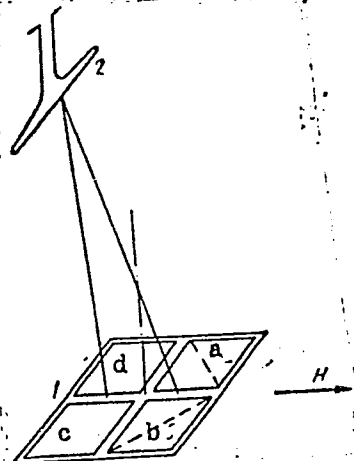
Fig. 1. Relative position of the base plate holder (1), evaporator (2), and external magnetic field (H).
