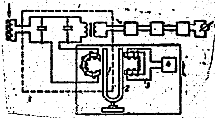
Fig. 1. 1 and 2- tuning fork prongs; 3- energizing system; 4- pumping oscillator
