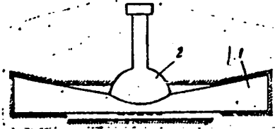
Fig. 1. 1 - radiator; 2 - photomultiplier
