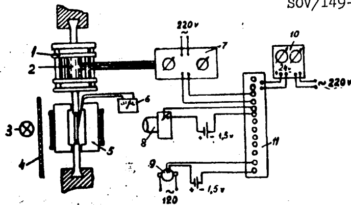
Fig. 1. Diagram of installation for simultaneous determination of applied force and cross section of the specimen during stretching. (1) Reverser; (2) dynamometer; (3) light source; (4) screen; (5) resistance heat; (6) galvanometer and thermocouple; (7) power supply; (8) photographic camera "Zenit-S"; (9) time recorder; (10) oscillograph rectifier; (11) oscillograph POB-14.
