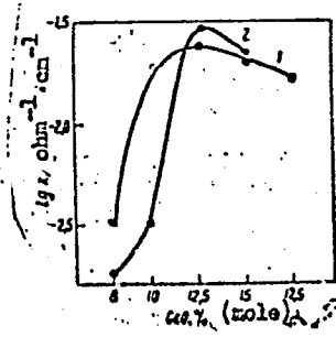
Fig. 2. Electroconductivity as a function of CaO content. Stabilizer in form of \text{CaCO}_3 (1) and \text{CaZrO}_3 (2)
