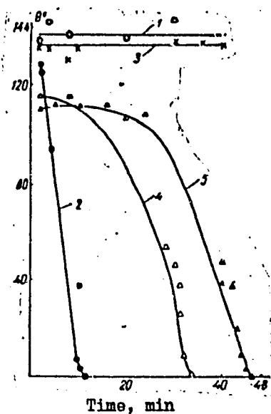
Fig. 2. Change in the contact angle as a function of time during wetting of Ti specimen oxidized in air at 800C by Ag-Cu alloy. Duration of oxidation in min and oxidation temperature respectively: 1 - 30, 800C; 2 - 30, 900; 3 - 60, 800; 4 - 60, 900; 5 - 120, 900.
