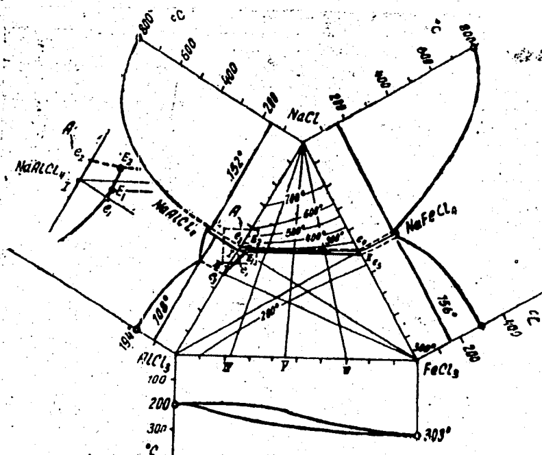
Fig. 1 Fusibility diagram of the AlCl_3 - FeCl_3 - NaCl System
