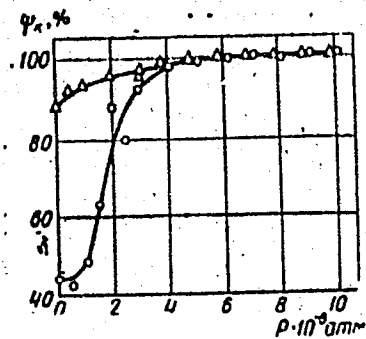
Fig. 1. Ductility of sound (1) and defective (2) specimens of N2 copper versus hydrostatic pressure
