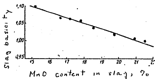
Fig. 3. The relationship between MnO contents in slag and its basicity ( \text{CaO}:\text{SiO}_2 ).
