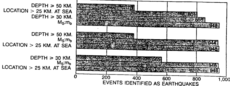
METHODS OF DISTINGUISHING earthquakes from explosions were tested by applying the methods to all the earthquakes with a magnitude of 4.5 or more recorded during a 162-day period in 1972. The sample consisted of 948 events. Many of them could be classified as earthquakes (rather than explosions) by their location or their depth. The remaining events could be classified by comparing the magnitude of long-period surface waves with the magnitude of short-period body waves (the ratio M_S:m_b ). The sequence in which the tests were applied affected the efficiency of the procedure, but all events were identified regardless of the sequence.
