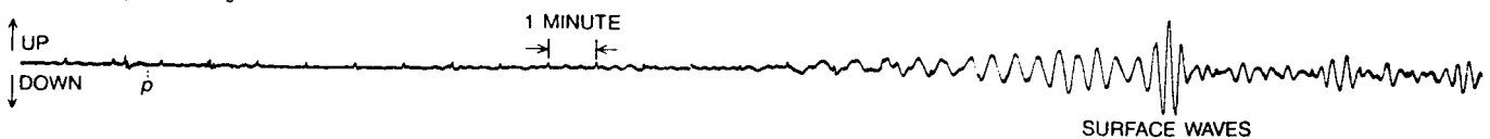
NUCLEAR EXPLOSION, U.S.S.R. AUGUST 28, 1972 m_b=6.3
