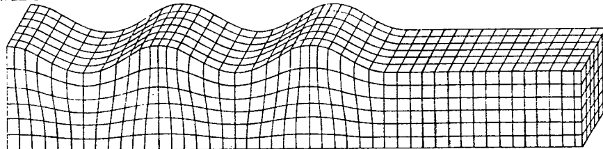
RAYLEIGH WAVE
