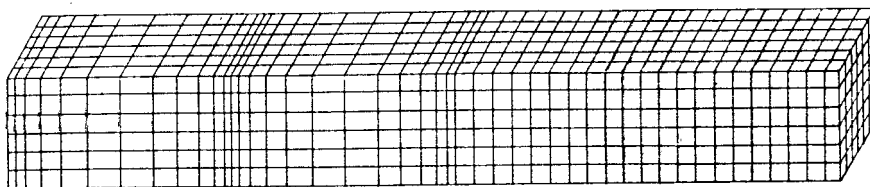
P WAVE
