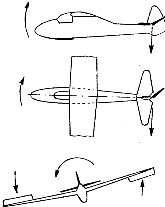
Sl. 71. — Krmila letala
