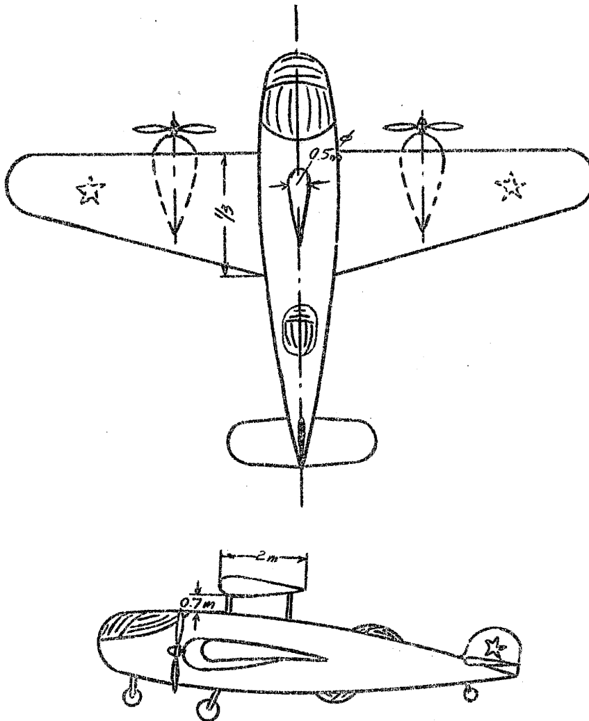
Sketch 5: Twin-Engine Aircraft Fitted with an Auxiliary Power Plant Observed in Moscow-Khimki
