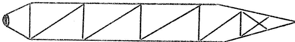
Sketch 2: Side View of Air-Frame Tubings
