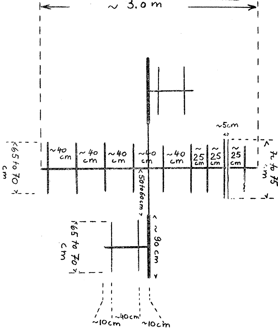
Top View of Eberswalde Radar Set
