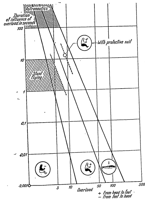
Allowable inertia overloads depend on position of man and duration of action of overload.
