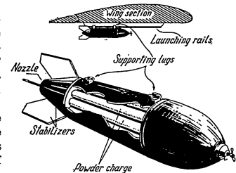
Plan of an aviation reaction projectile.
