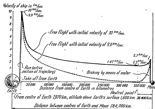
Graph of flight: Earth-Moon.
