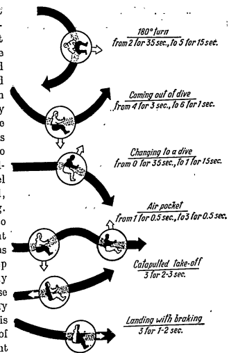
Inertia overloads acting on pilot during flight.
