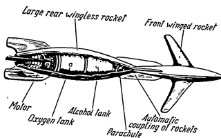
Step-rocket (project).
