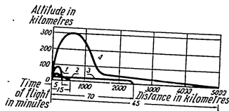
Trajectory of flight of various long-range rockets: 1—initial long-range rocket described in Chapter 6; 2—the same rocket equipped with wings; 3, 4—step-rocket.
