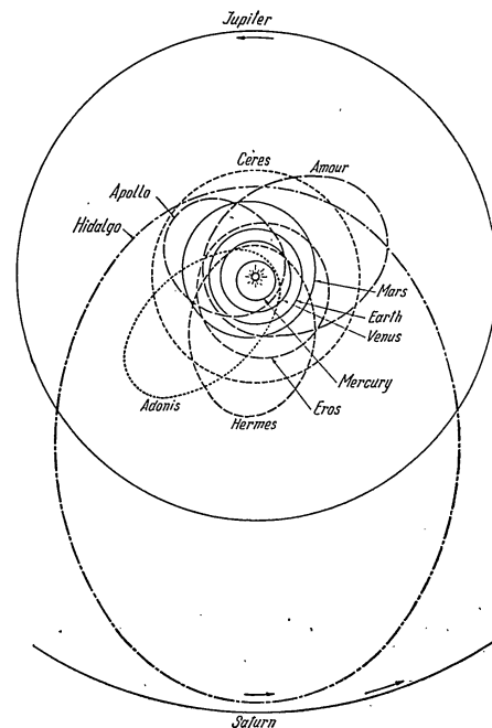
Orbits of certain asteroids.
