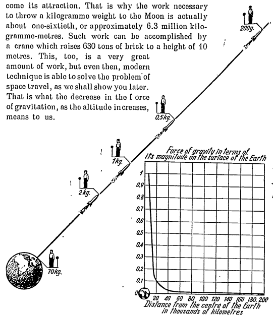
The force of gravity is inversely proportional to the square of the distance from the centre of the Earth.
