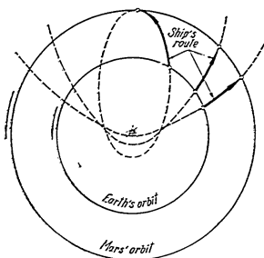
Trajectories of express flights: Earth-Mars.
