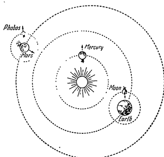
"Reconstruction" of the solar system.
