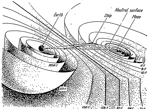
In the field of gravitation of the Earth and the Moon, Surfaces are shown, on any point of which the ratio of the forces of attraction to the Earth and the Moon is identical (indicated by figures).
