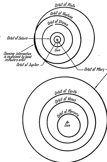
Above is shown the scheme of the solar system on scale where 1 mm. is equal to one astronomical unit (astronomical unit—distance from the Earth to the Sun—is equal to 149.5 million kilometres). Using this scale, we can show the orbits of only the five so-called outer planets, beginning with Jupiter. Below we show, on an enlarged scale, the scheme of the central part of the solar system with the orbits of the inner planets. The increase in scale is seen from the orbit of Mars, as given in both schemes.
