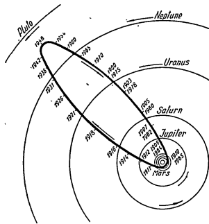
Path of Halley's comet in the solar system.
