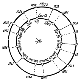
Oppositions of Mars from 1939 to 1971.
