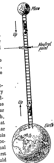
"Travel" from the Earth to the Moon.
