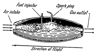
Scheme of uniflow air-reaction motor.
