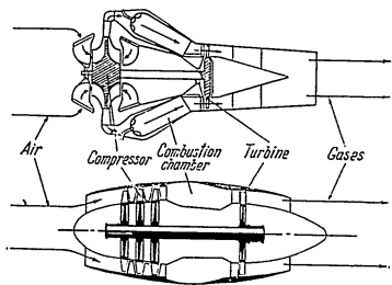
Schemes of turbo-reaction motors: above—with centrifugal compressor; below—with axial.
