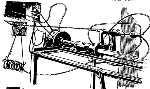
F. Tsander's liquid-fuel rocket motor on test stand (1933).
