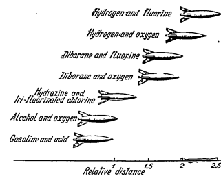
Relative distance of flight of rockets operating on different fuels. The distance covered by a rocket working on gasoline and nitric acid is taken as the unit.
