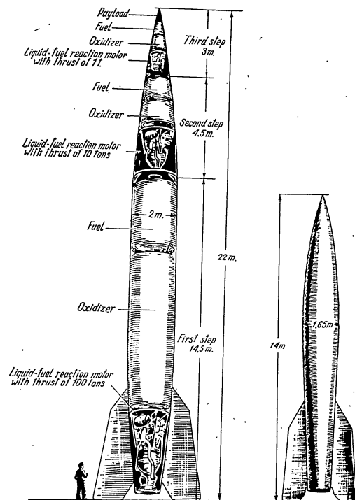
Three-step rocket for sending a load of 10 kg. to the Moon. At right—long-range rocket described in Chapter 6.
