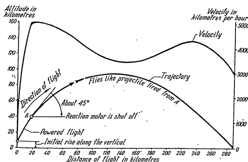
Trajectory and velocity of rocket flight.
