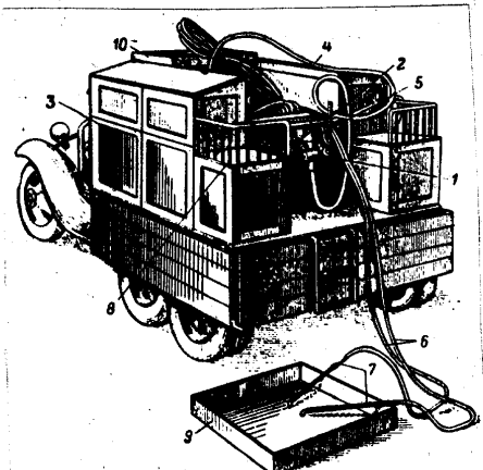
Figure 13. ADM-750 Auto-degasification machine. 1, hand pump; 2, barrel; 3, chest of drawers; 4, siphoning hose; 5, pressure hose; 6, distribution hoses; 7, nozzles; 8, seats; 9, receptacle which can be removed from the machine; 10, receptacle on the machine.
