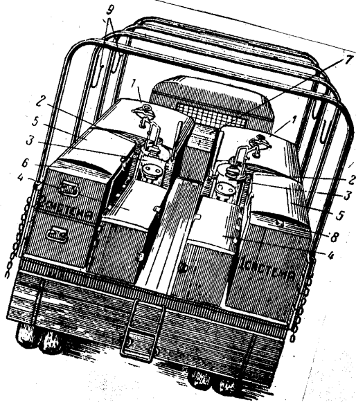
Figure 10. ADM-48 Auto-degasification machine. 1, tank; 2, distributing tank; 3, hand pump; 4, small case; 5, large case; 6, tool chest; 7, case for dose measuring instruments; 8, barrel (receptacle) for dichlorethane; 9, hooks for coiling the rubber and metal hoses.
