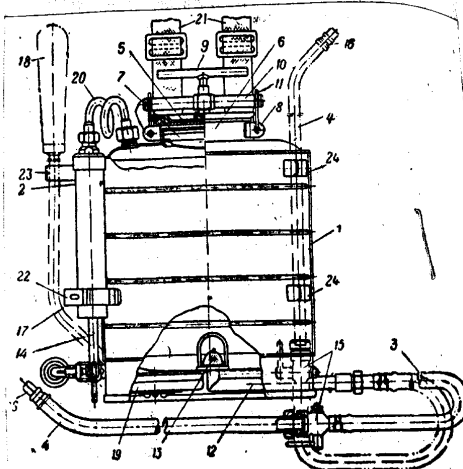
Figure 6. Portable degasification instrument, RDP-4 type. 1, tank; 2, air pump; 3, hose; 4, nozzle; 5, cover; 6, opening; 7, screen; 8, filter; 9, holders; 10, support screw; 11, beam; 12, clamp; 13, drainage pipe; 14, mobile filter; 15, piston; 16, sprayer;
