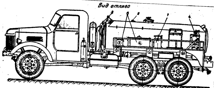
Figure 15. The ARS-12 automobile filling station. 1, tank; 2, pipes; 3, mechanical pump; 4, hand pump; 5, portable degasification instrument; 6, instrument and spare part chests; 7, vessel for liquid degasifying substance; 8, blind nut of the connecting pipe cutting off the siphon; 9, blind nut of the filling indicator.
