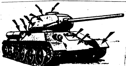
Figure 23. Parts of a tank which must be processed with partial degasification, deactivation, and disinfection.
