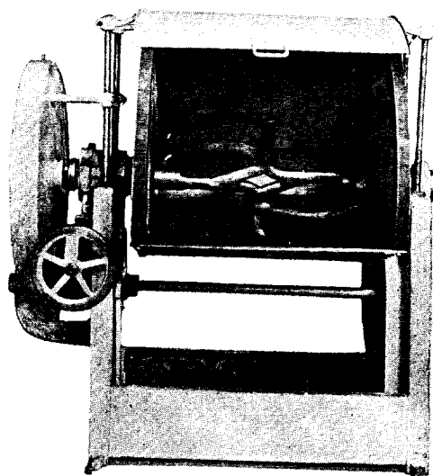
BISCUIT DOUGH MIXER MEDIUM SIZE
