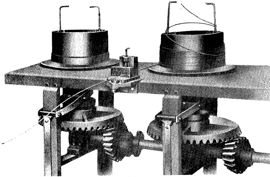
(A) WIRE DRAWING MACHINE (ARRANGED IN SERIES)
