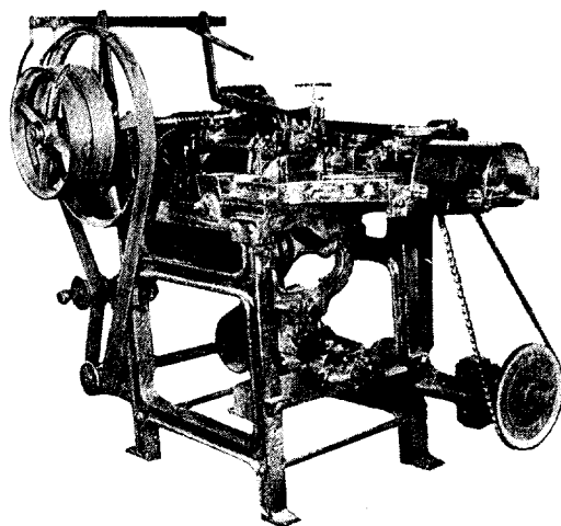
WIRE STRAIGHTENING, CUTTING & SHARPENING MACHINE ITEM 1.
