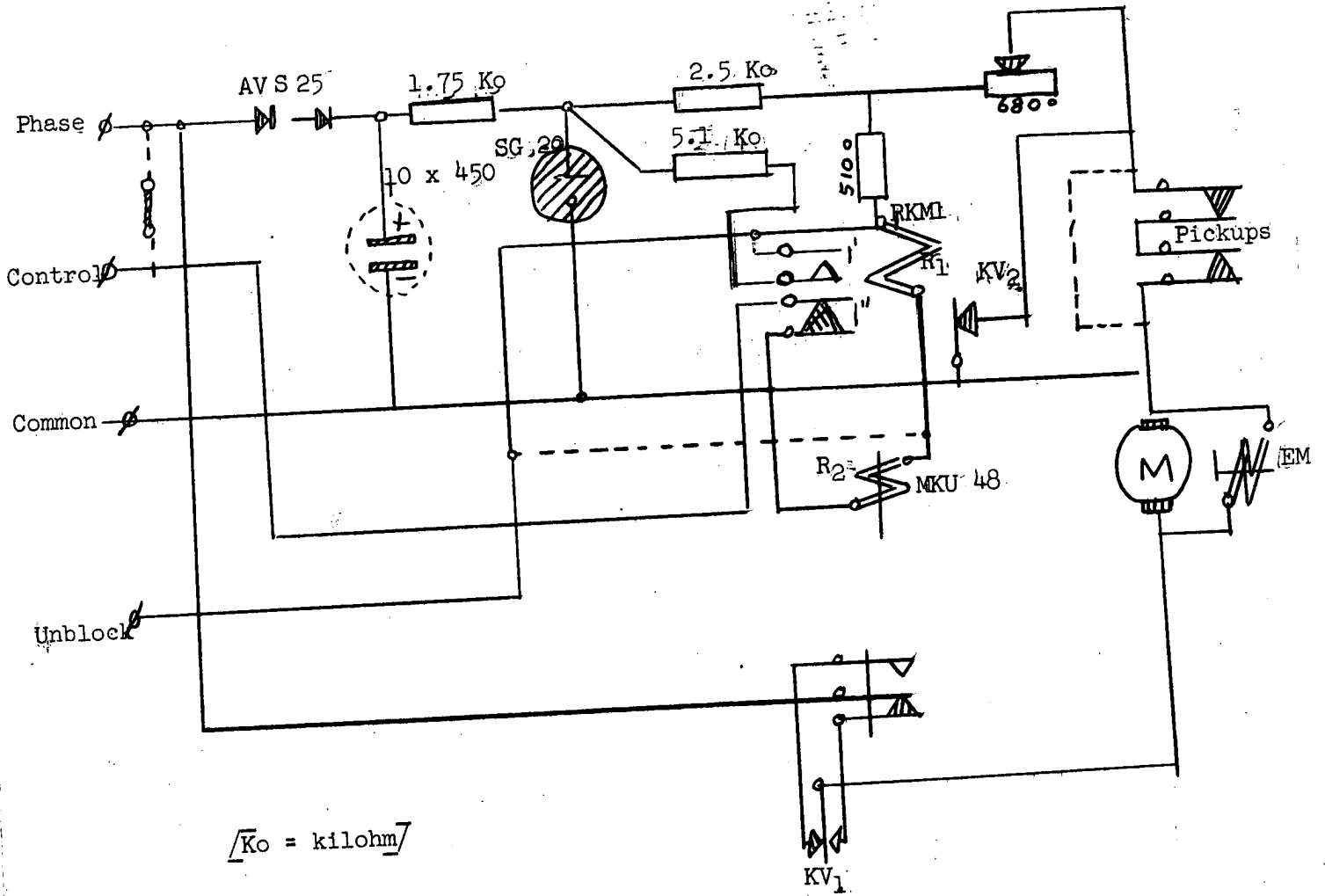
Fig. 9. Basic diagram of operation of the EFM-2 with the electrified PS-54 sighting device (dotted lines indicate modifications).
