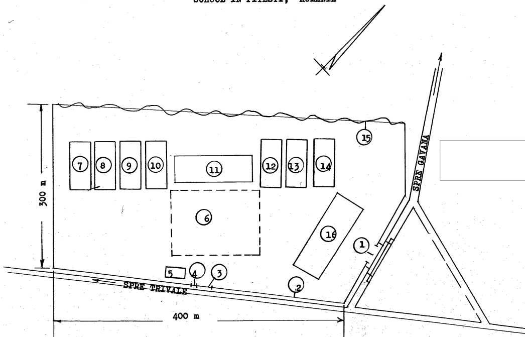
SKETCH OF CASERN OCCUPIED BY UNIDENTIFIED ARMORED OFFICERS' SCHOOL IN PITESTI, RUMANIA
