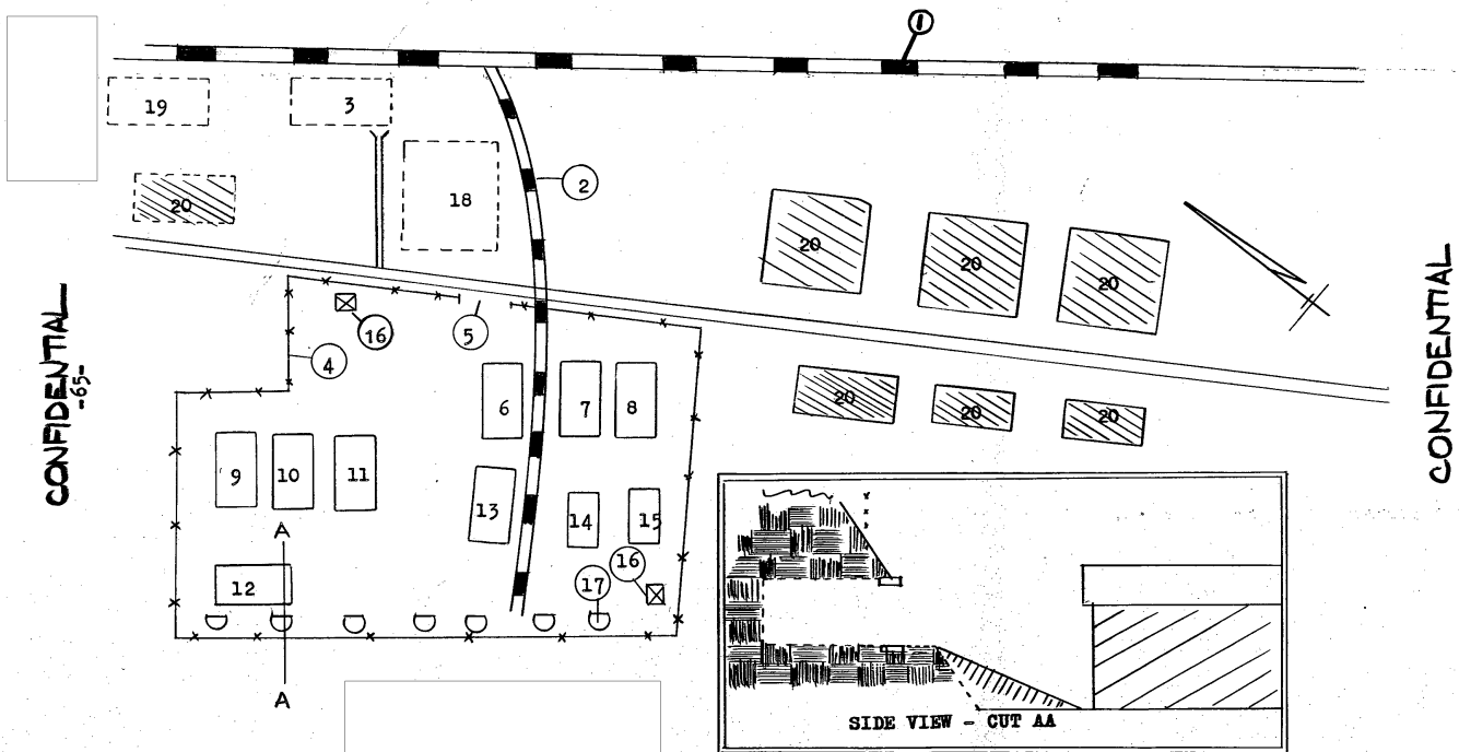
SKETCH OF CASERN OCCUPIED BY UNIDENTIFIED ENGINEER REGIMENT AND LOCATION OF AN UNDERGROUND AMMUNITION STORAGE AREA IN BASCOV, ROMANIA
