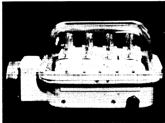
Large pod of infrared tracking light used for tracking missiles against the stars.
