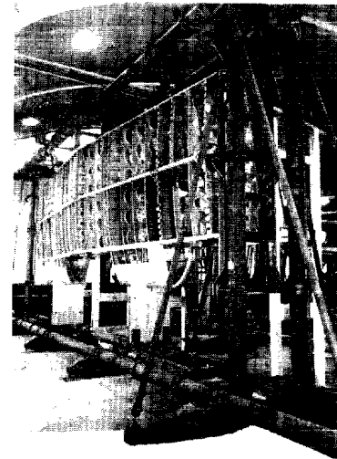
The structural design of the wing with three spurs appears from this picture
