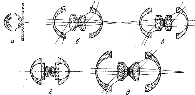
Fig. 10 - Various Kinds of Aerial Survey Objectives. ("Razlichnyye Vidy Aeros"yemochnykh Ob"yektivov.").
