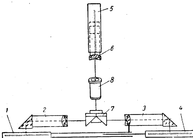
Fig. 2 - Design of the Optical Lay-out for Readings of Coordinates and Parallaxes in the "Naklonnyy Stereokomparator", (Oblique Stereocomparator).
