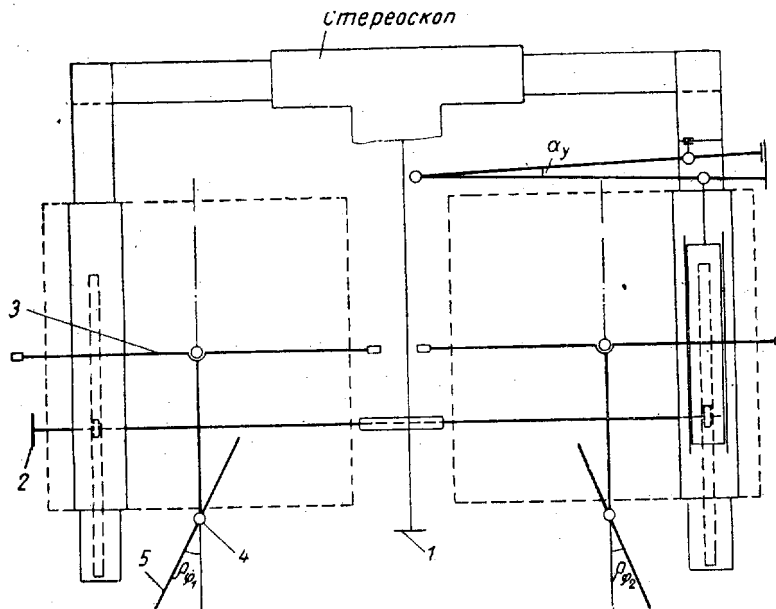
Fig. 9 - Design of Kern Stereometer. ("Skhema Kern-Stereometra").
