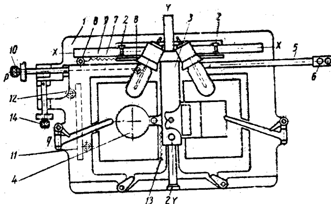
Fig. 5 - Working Parts of the Drobyshev Stereopantometer SPD-1.
