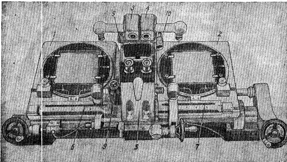
Fig. 1 - Oblique Stereocomparator ("Naklonnyy Stereokomparator")
