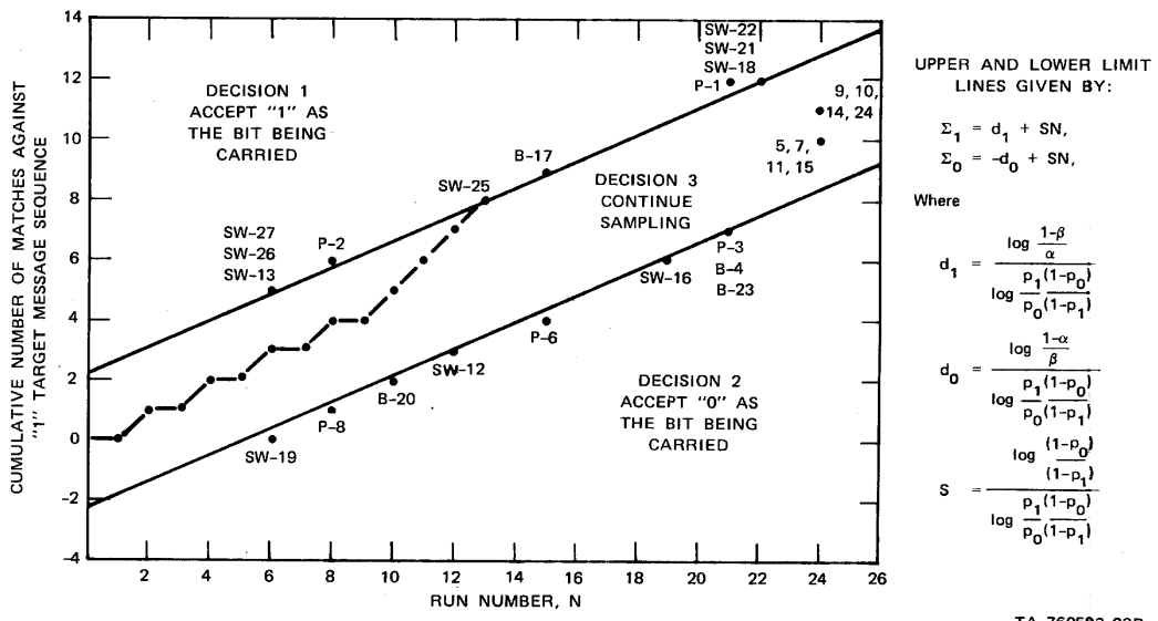
FIGURE 10 PROCEDURE FOR CARD SORTING BY SEQUENTIAL SAMPLING p_0 = 0.324, p_1 = 0.564, \alpha = 0.1, \beta = 0.1 BROKEN LINE SHOWS SAMO SAMPLING SEQUENCE FOR CARD NO. 25
