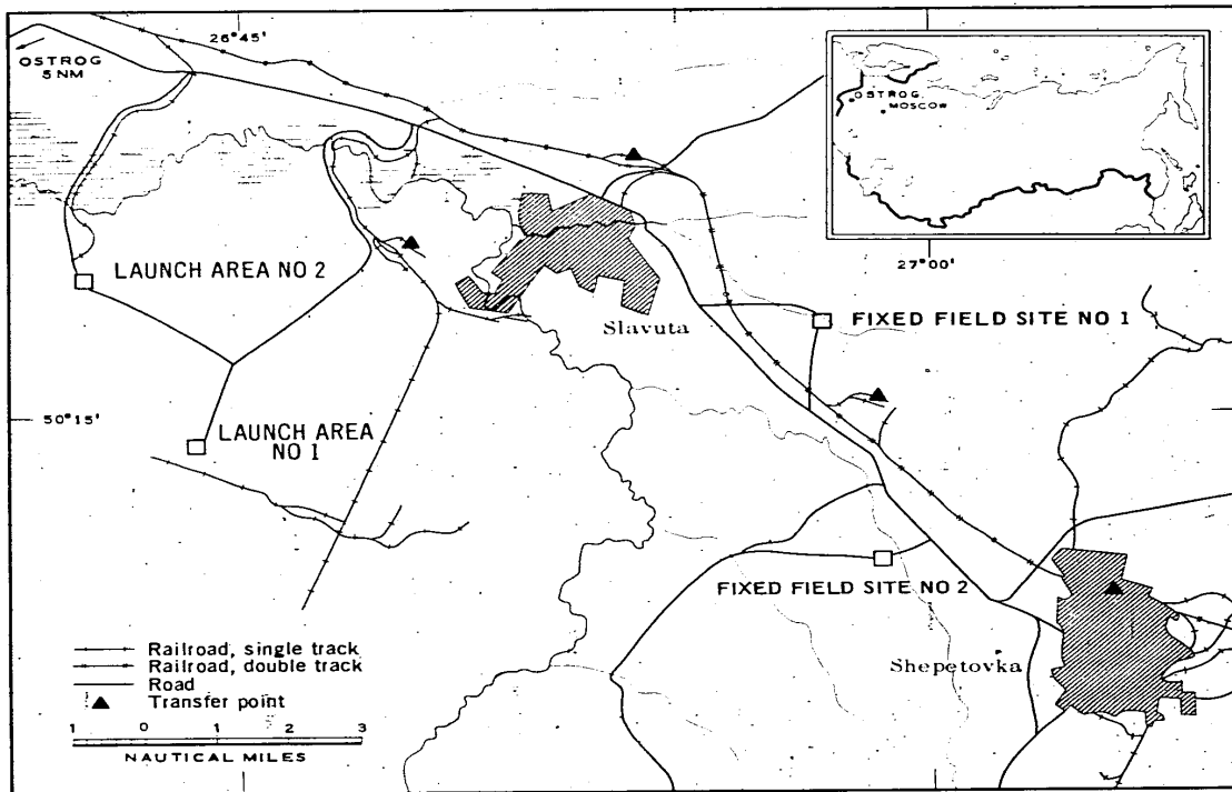
FIGURE 1. OSTROG MRBM COMPLEX, USSR.
