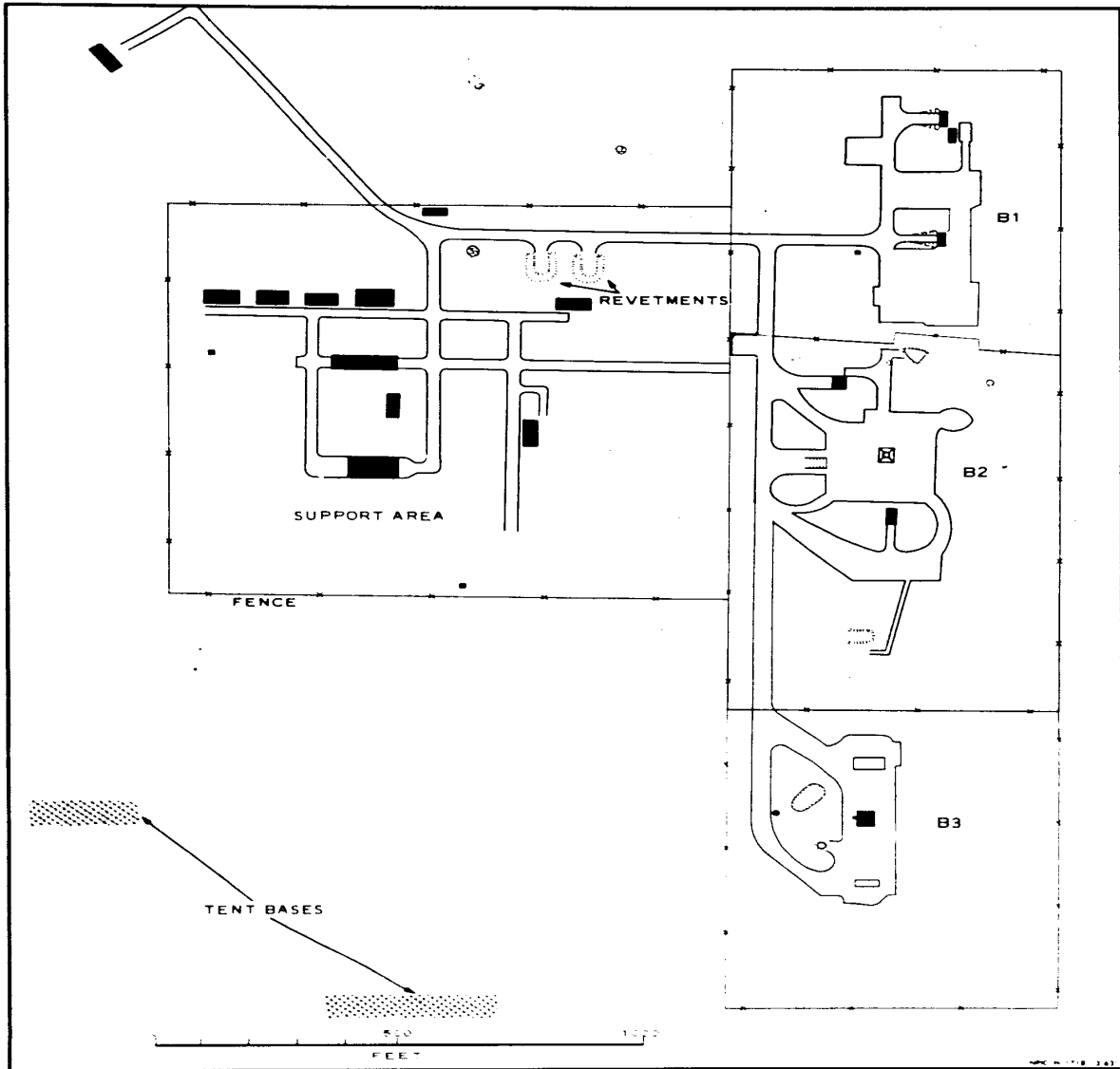
FIGURE 5. LAUNCH COMPLEX B.
