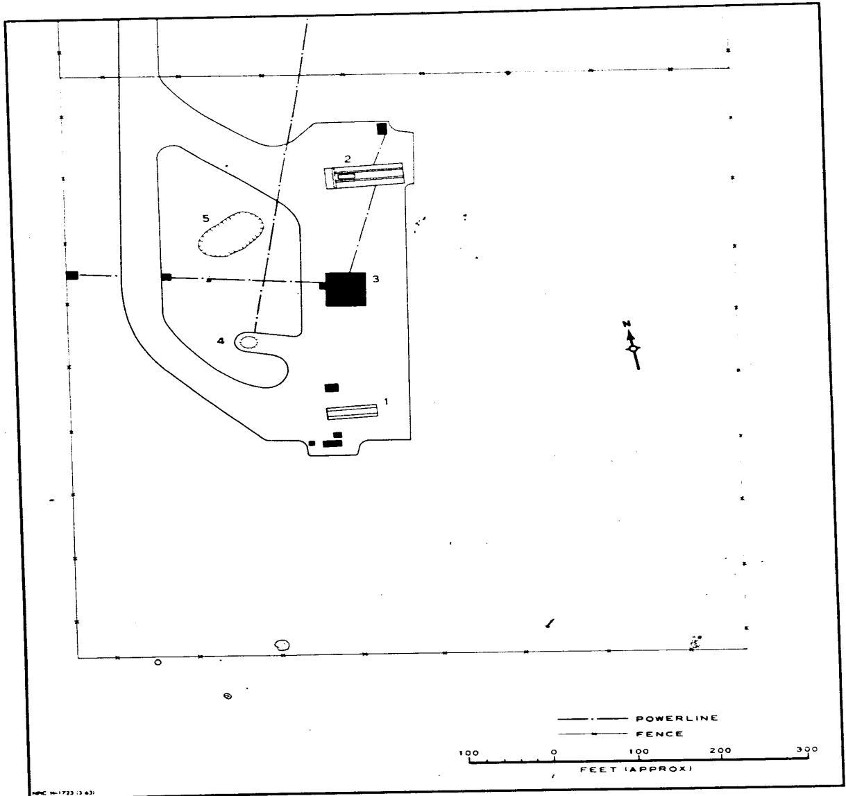
FIGURE 10. LAUNCH AREA B3.
