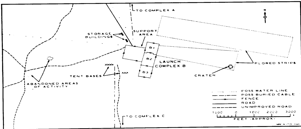
FIGURE 2. GENERAL AREA OF LAUNCH COMPLEX B.
