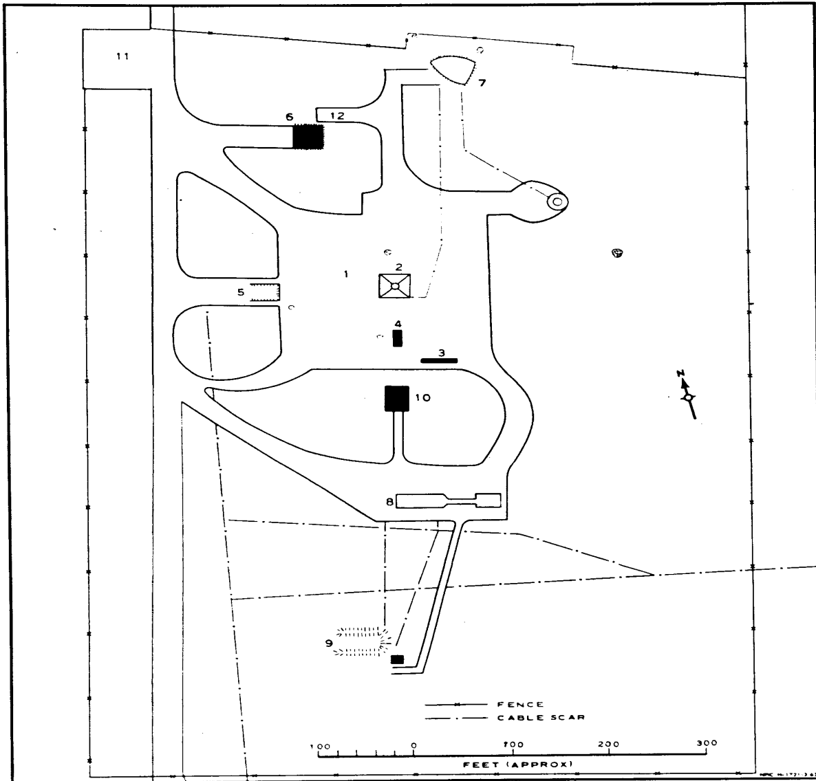
FIGURE 8. LAUNCH AREA B2.
