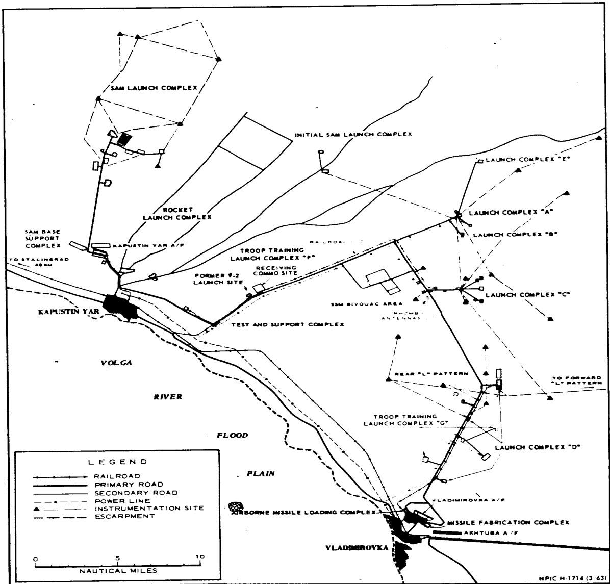
FIGURE 1. KAPUSTIN YAR VLADIMIROVKA MISSILE TEST CENTER.
