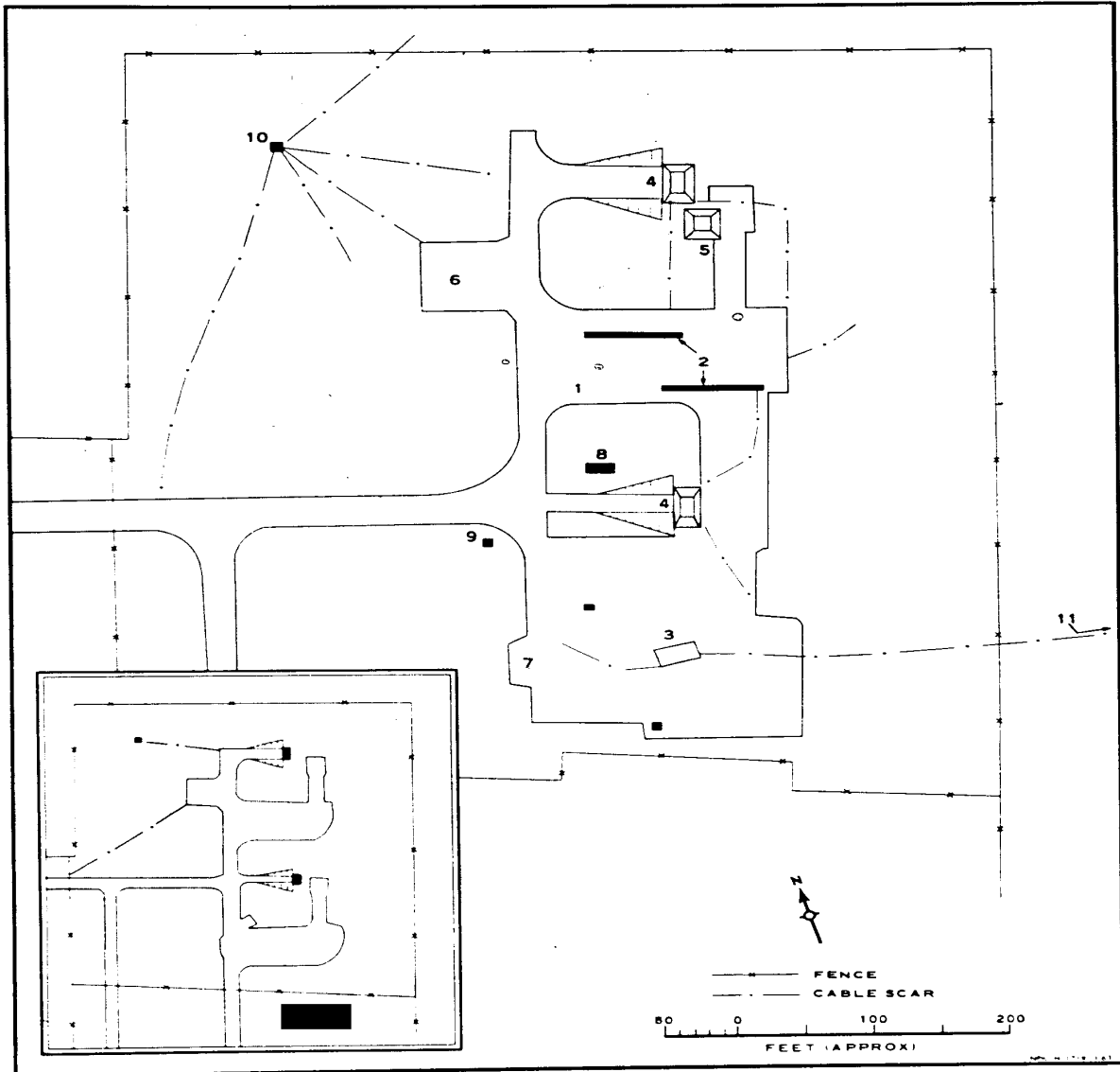
FIGURE 6. LAUNCH AREA B1.
