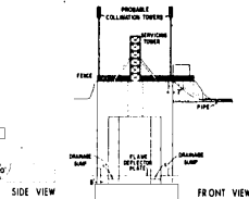
LAUNCHING STRUCTURE
